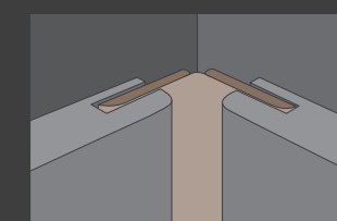
Flexible moulding FAL Folded inwards for covering the transitions on dormer windows and pitched roofs
