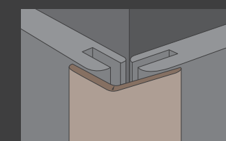
Flexible moulding FAL Foldable moulding for neat transitions on non-rightangled connections
